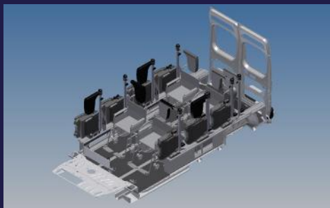
Full wheelchair (above & left) 2 wheelchairs, 4 seats (right)
