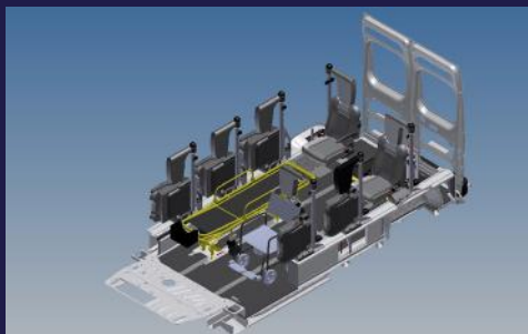
Stretcher, wheelchair & 2 seats (above & left), stretcher, wheelchair & 3 seats (right)
